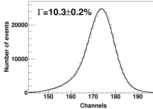
Fig.6. Amplitude spectrum of events recorded by \alpha -pixel 3 without coincidence with the signal from the gamma-detector.
