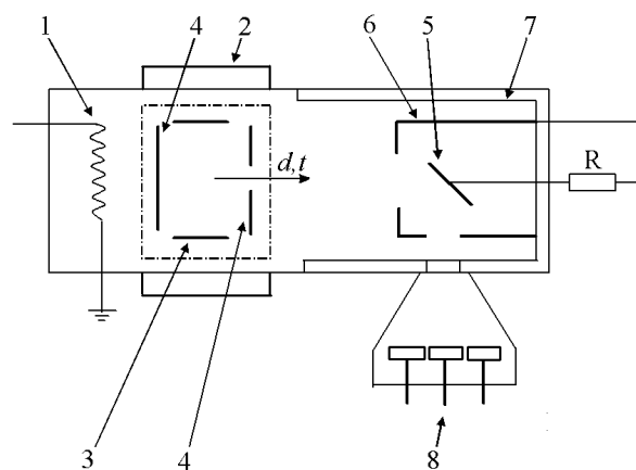
Fig.1. Schematic view of the gas-filled neutron tube with the \alpha -detector.
