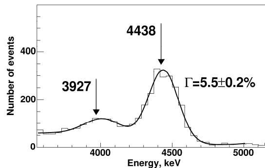
Fig.7. Energy spectrum of events recorded by the gamma-detector (in coincidence with the signal from alpha-pixel 3) in irradiation of a ^{12}\text{C} sample with a tagged neutron flux.
