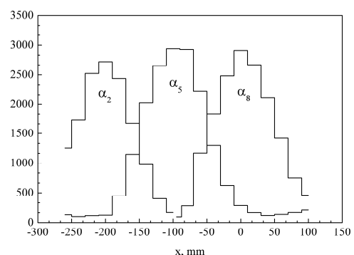
Fig.5. Spatial neutron distribution in tagged beams corresponding to alpha-detector pixels 2,5 and 8 (along the X axis)
