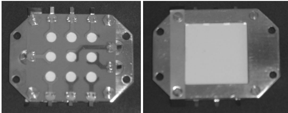
Fig.3. 9-pixel alpha-detector viewed from the back and from the tritium target side.
