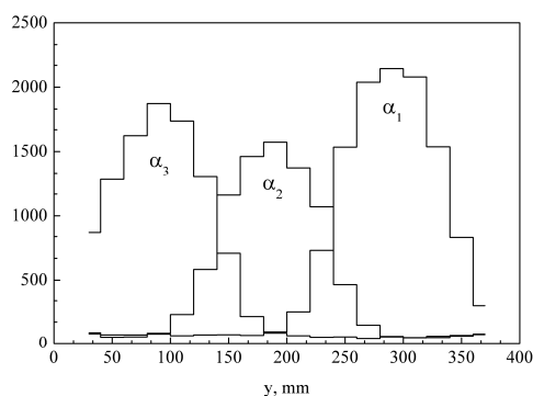
Fig.4. Spatial neutron distribution in tagged beams corresponding to alpha-detector pixels 1,2 and 3 (along the Y axis)
