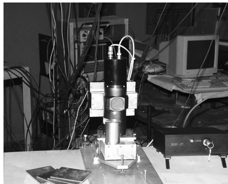
Fig.2. Portable neutron generator with a 9-pixel \alpha -detector
